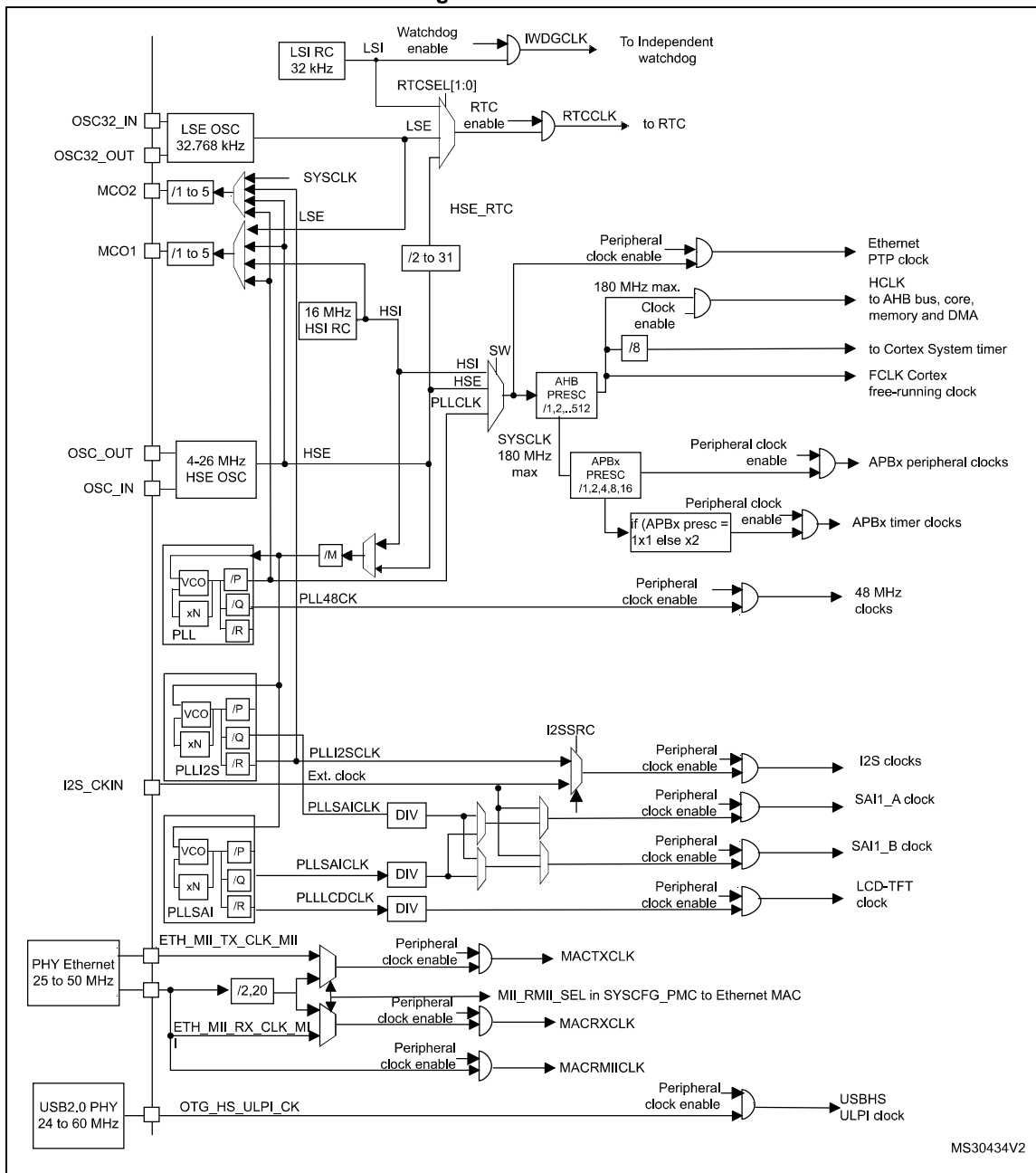
Figure 16. Clock tree
